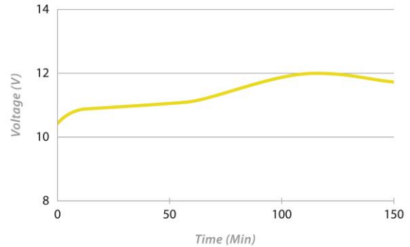
CHARGE CHARACTERISTICS
